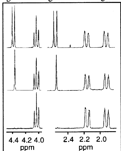
Figure 2 : ^1H -NMR ( CHCl_3 ) selected regions for (X, B,K) complexes: X = 1 (top), X = 2 (middle), X = 3 (bottom)
