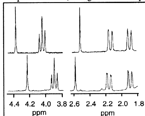
Figure 3 : ^1H -NMR ( CHCl_3 ) selected regions, (2, B,M) complexes: M = K^+ (top), M = Cs^+ (bottom)
